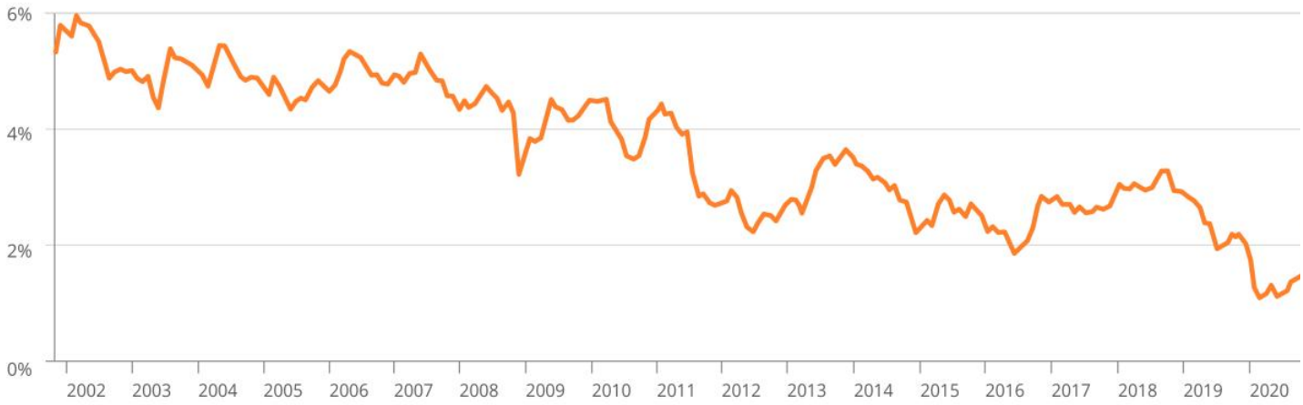
U.S. Government 20-Year Treasury Yields: 10/1/01 - 9/30/21
